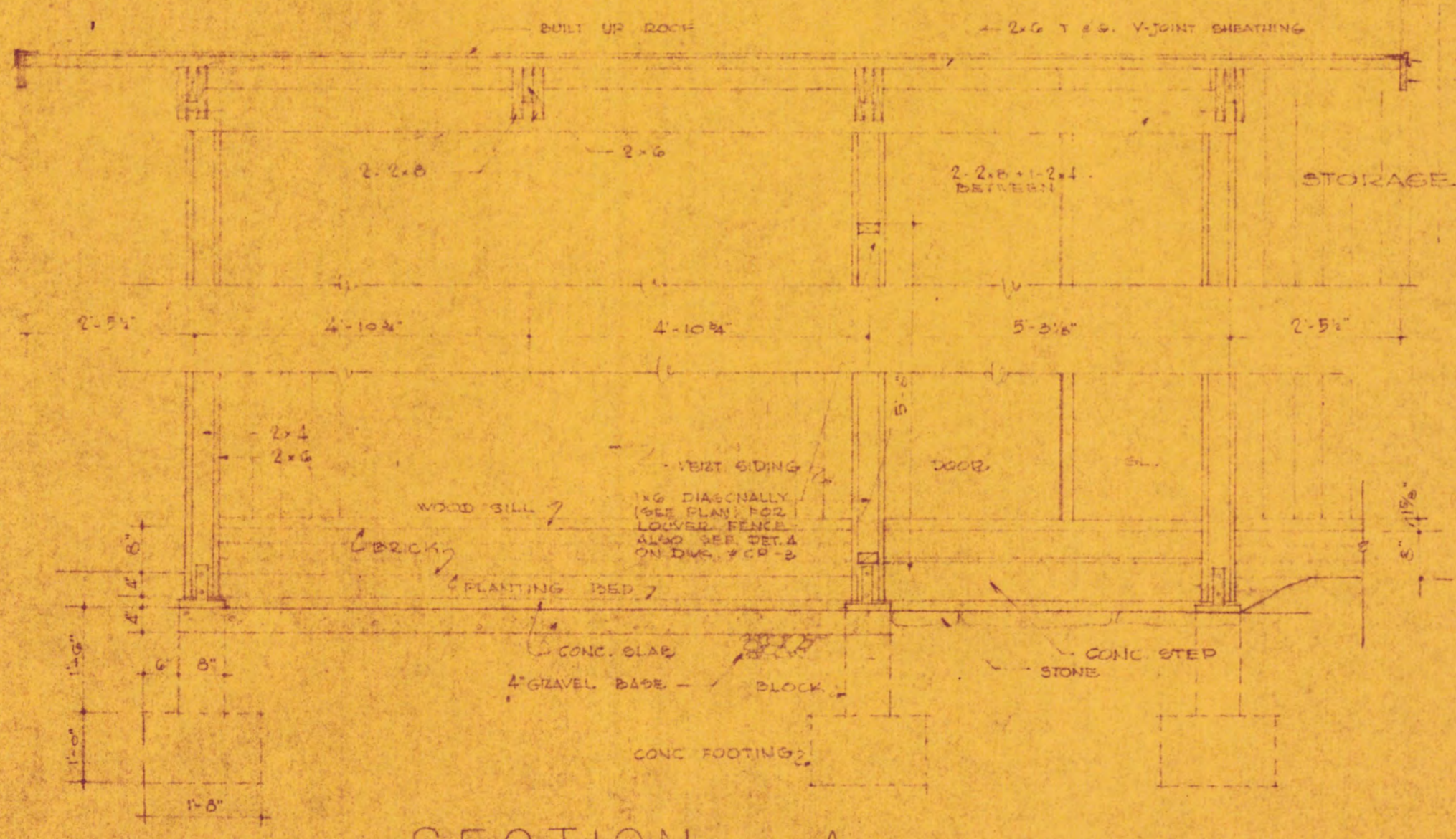
SECTION A 1/2" = 1'-0"
