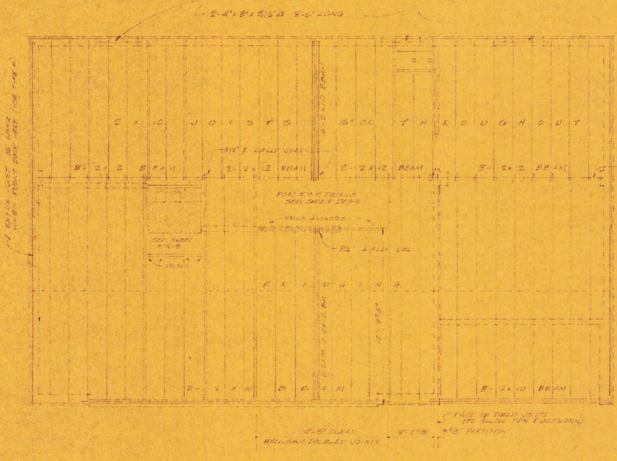
FLOOR FRAMING
