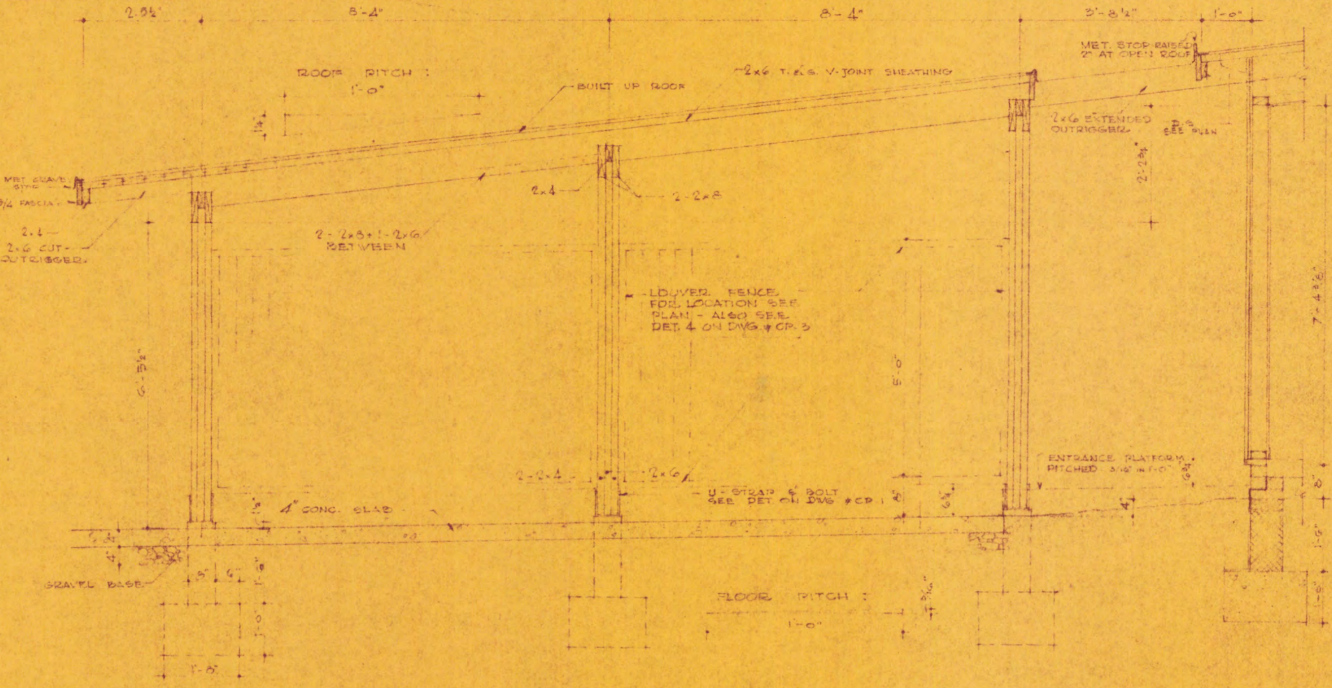
SECTION B 1/2" = 1'-0"
