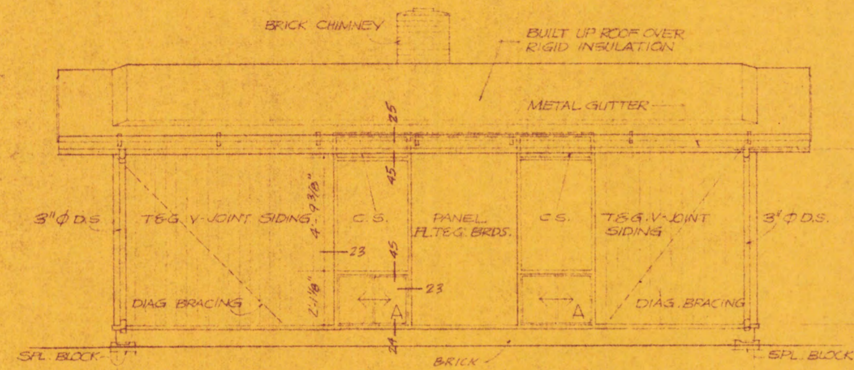
ELEVATION C
