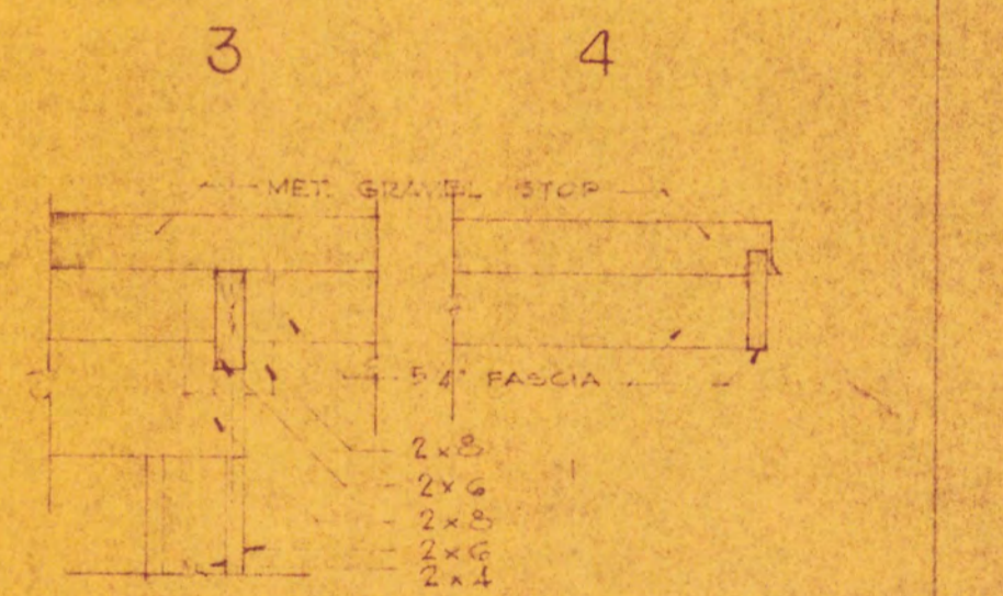
SECTION C 1" = 1'-0"
