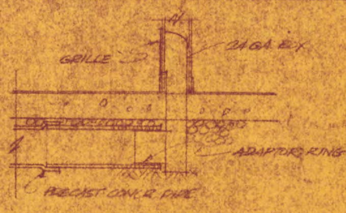
SECTION AT GRILLE
